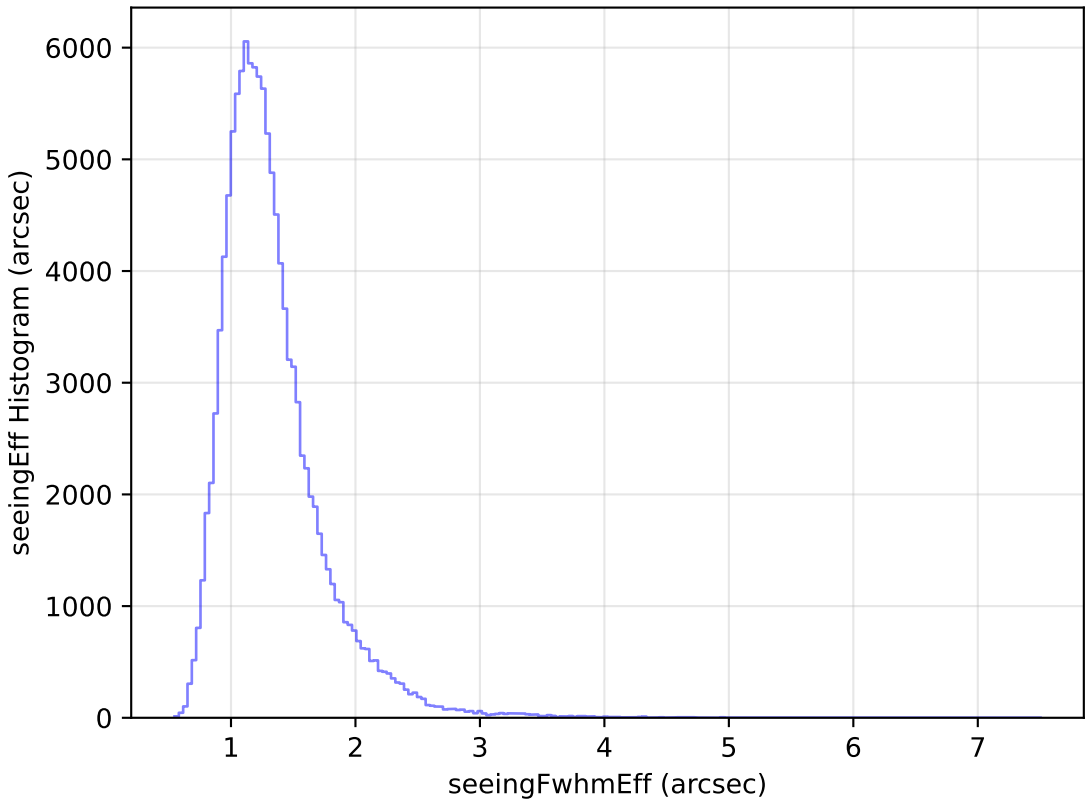
ddf_loaded_half_fl15_v3.4_10yrs WFD u band: seeingEff Histogram
