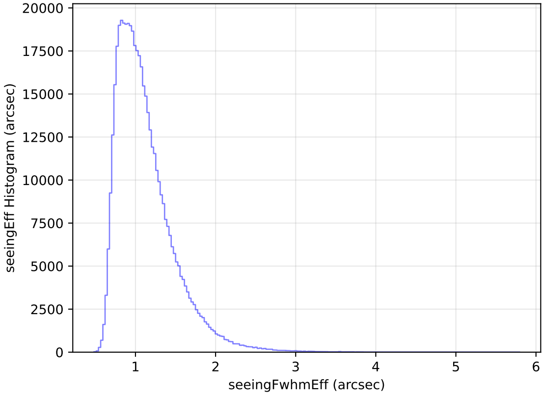
ddf_loaded_half_fl15_v3.4_10yrs WFD r band: seeingEff Histogram
