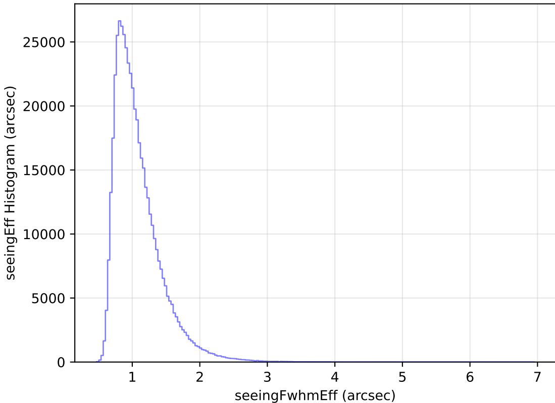
ddf_loaded_half_fl15_v3.4_10yrs WFD i band: seeingEff Histogram
