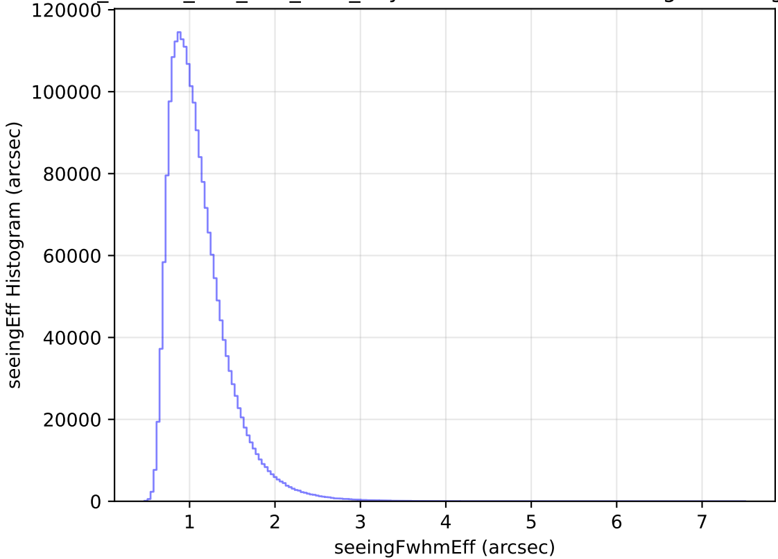
ddf_loaded_half_fl15_v3.4_10yrs WFD all bands: seeingEff Histogram
