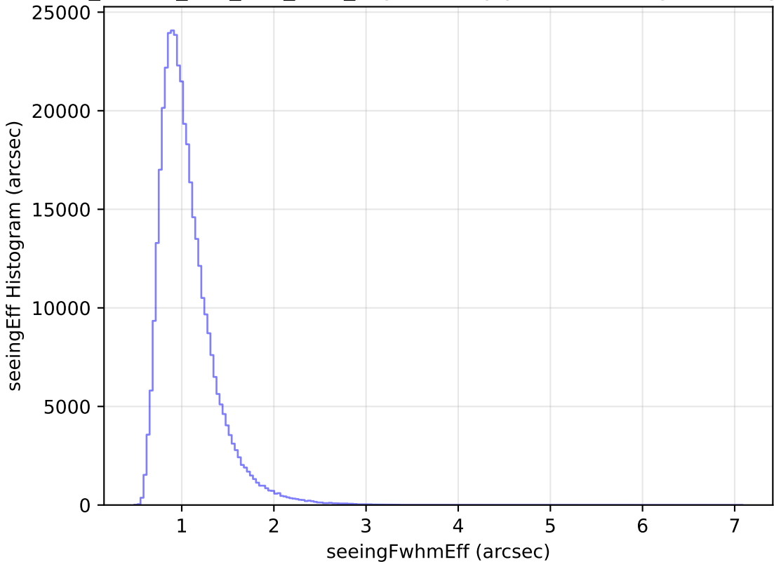
ddf_loaded_half_fl15_v3.4_10yrs All sky y band: seeingEff Histogram
