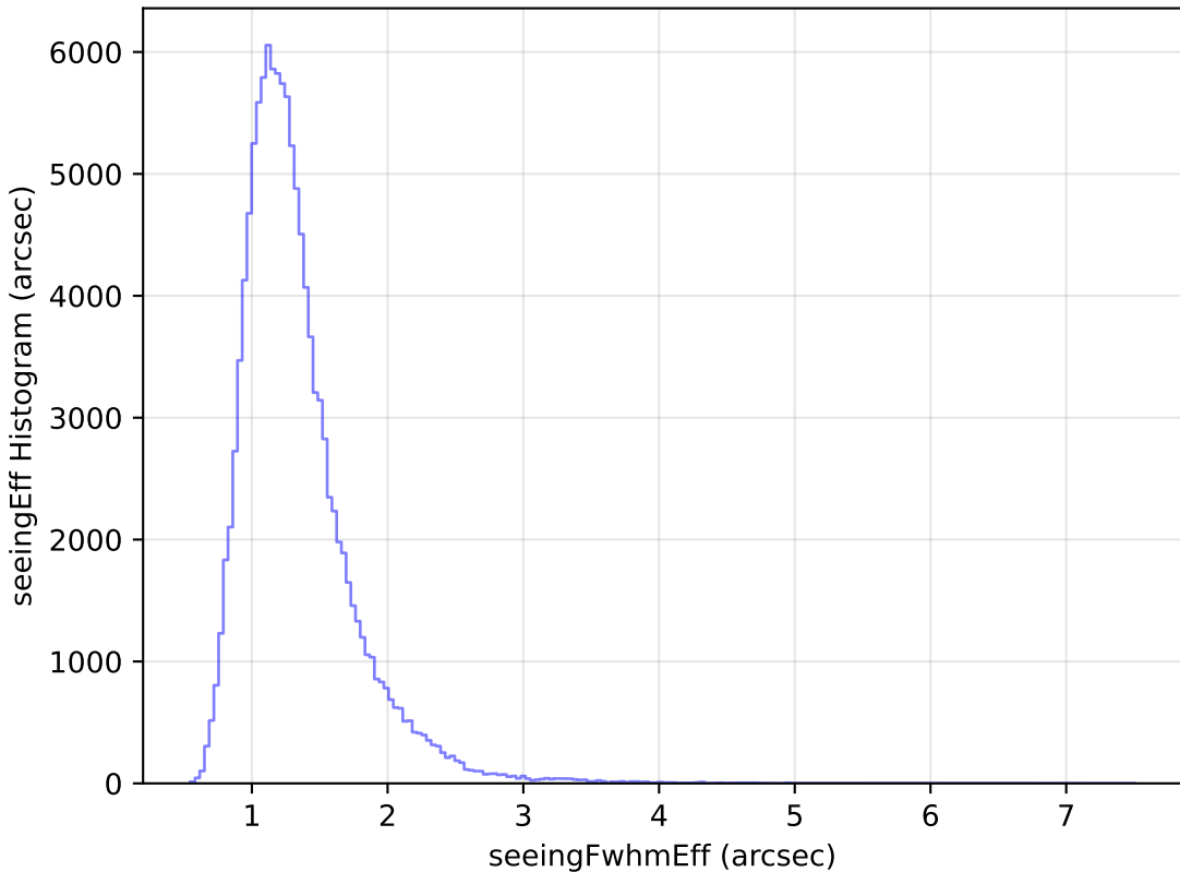
ddf_loaded_half_fl15_v3.4_10yrs All sky u band: seeingEff Histogram
