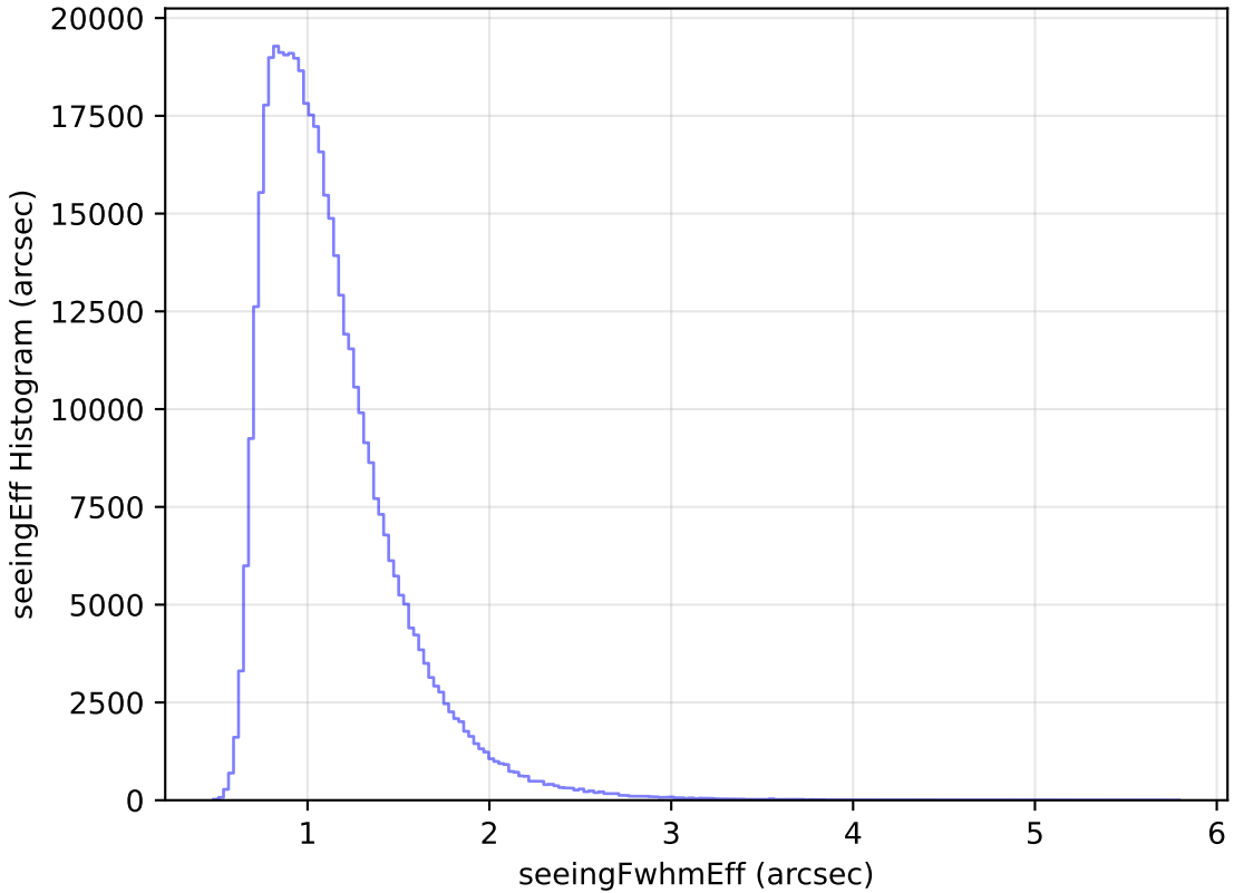
ddf_loaded_half_fl15_v3.4_10yrs All sky r band: seeingEff Histogram
