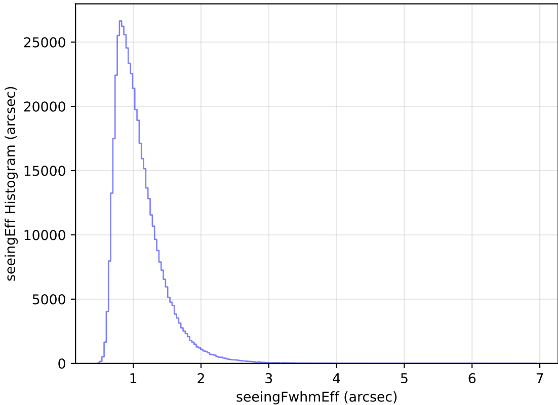
ddf_loaded_half_fl15_v3.4_10yrs All sky i band: seeingEff Histogram
