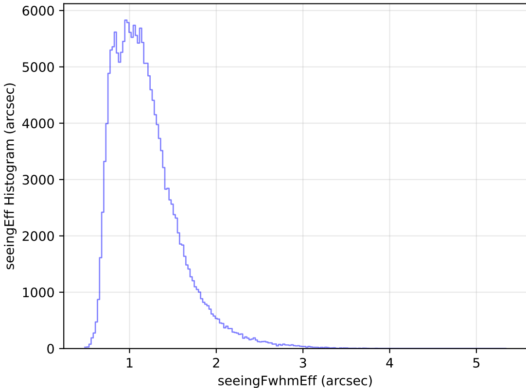
ddf_loaded_half_fl15_v3.4_10yrs All sky g band: seeingEff Histogram
