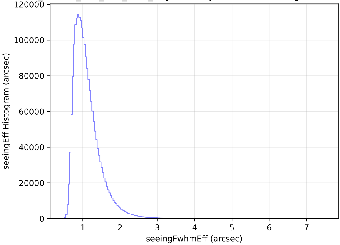
ddf_loaded_half_fl15_v3.4_10yrs All sky all bands: seeingEff Histogram
