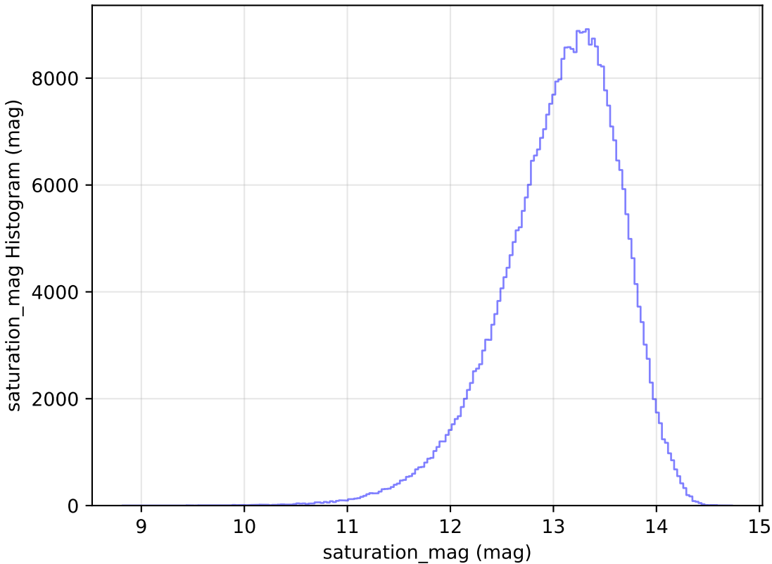
ddf_loaded_half_fl15_v3.4_10yrs WFD y band: saturation_mag Histogram
