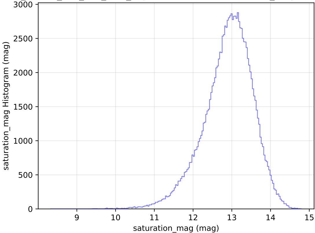
ddf_loaded_half_fl15_v3.4_10yrs WFD u band: saturation_mag Histogram
