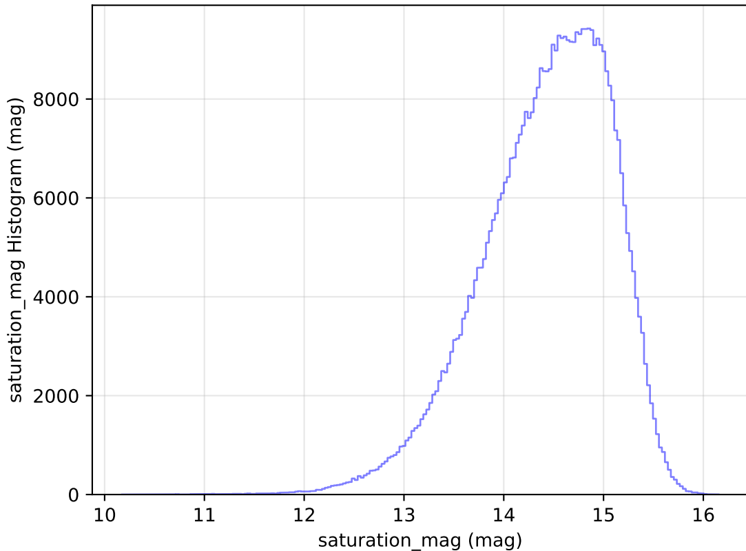
ddf_loaded_half_fl15_v3.4_10yrs WFD i band: saturation_mag Histogram
