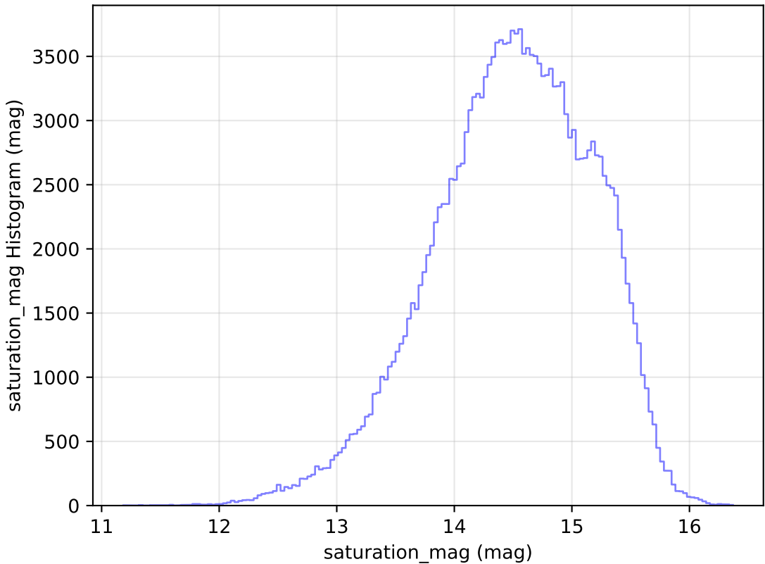
ddf_loaded_half_fl15_v3.4_10yrs WFD g band: saturation_mag Histogram
