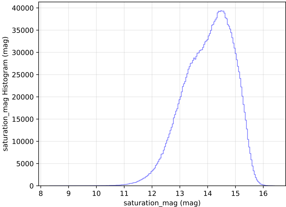
ddf_loaded_half_fl15_v3.4_10yrs WFD all bands: saturation_mag Histogram
