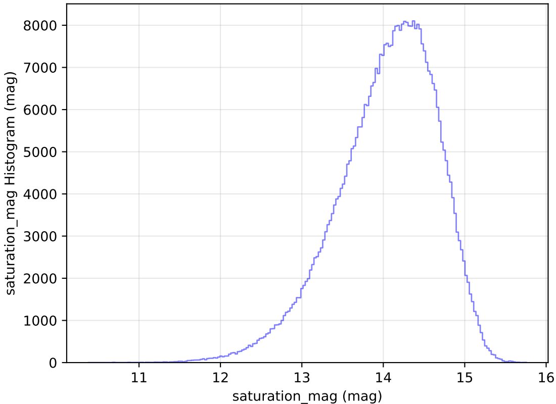
ddf_loaded_half_fl15_v3.4_10yrs All sky z band: saturation_mag Histogram
