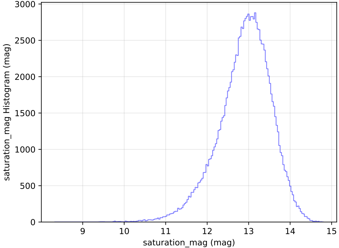
ddf_loaded_half_fl15_v3.4_10yrs All sky u band: saturation_mag Histogram
