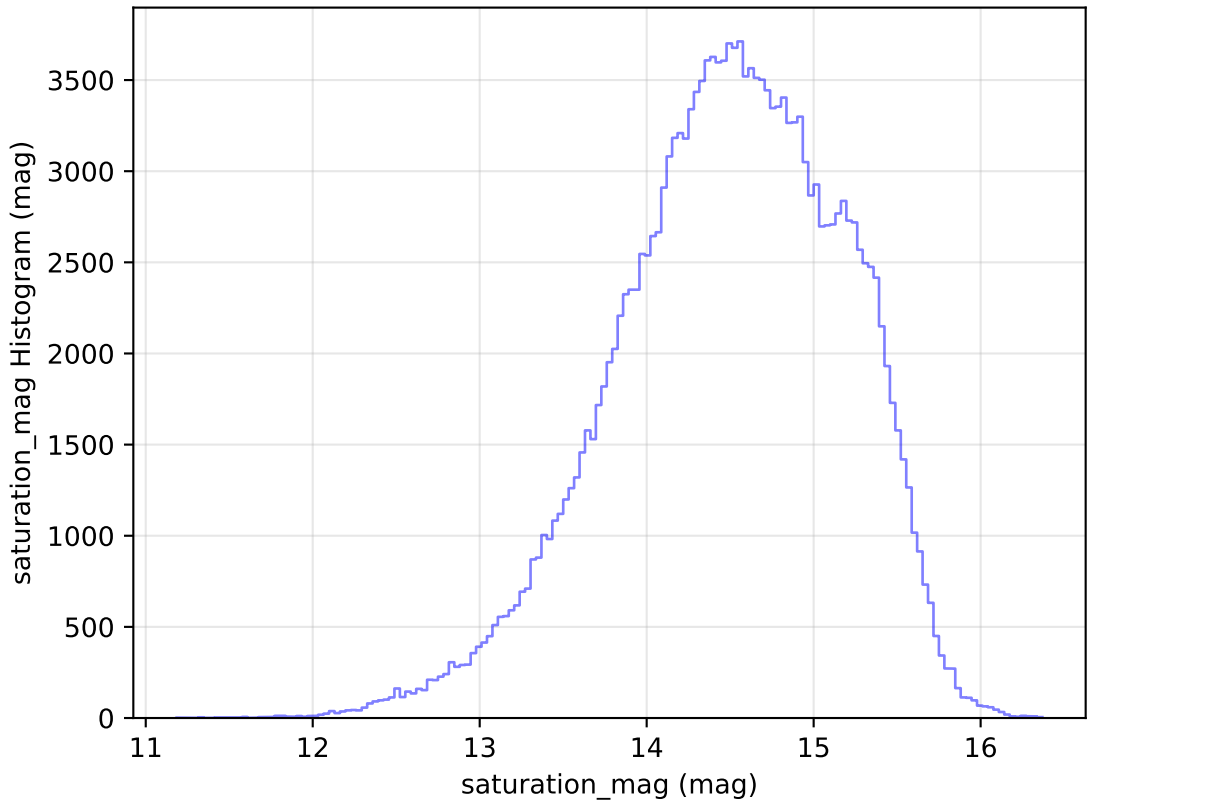
ddf_loaded_half_fl15_v3.4_10yrs All sky g band: saturation_mag Histogram
