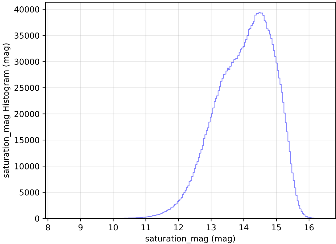
ddf_loaded_half_fl15_v3.4_10yrs All sky all bands: saturation_mag Histogram
