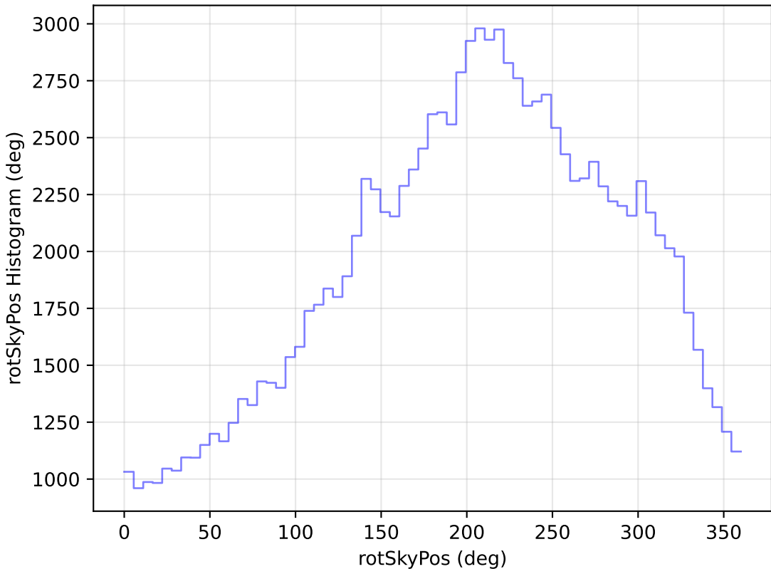
ddf_loaded_half_fl15_v3.4_10yrs WFD u band: rotSkyPos Histogram
