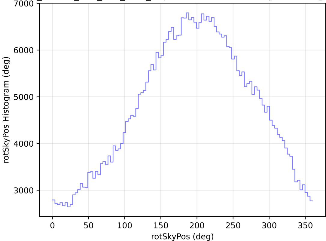
ddf_loaded_half_fl15_v3.4_10yrs WFD r band: rotSkyPos Histogram
