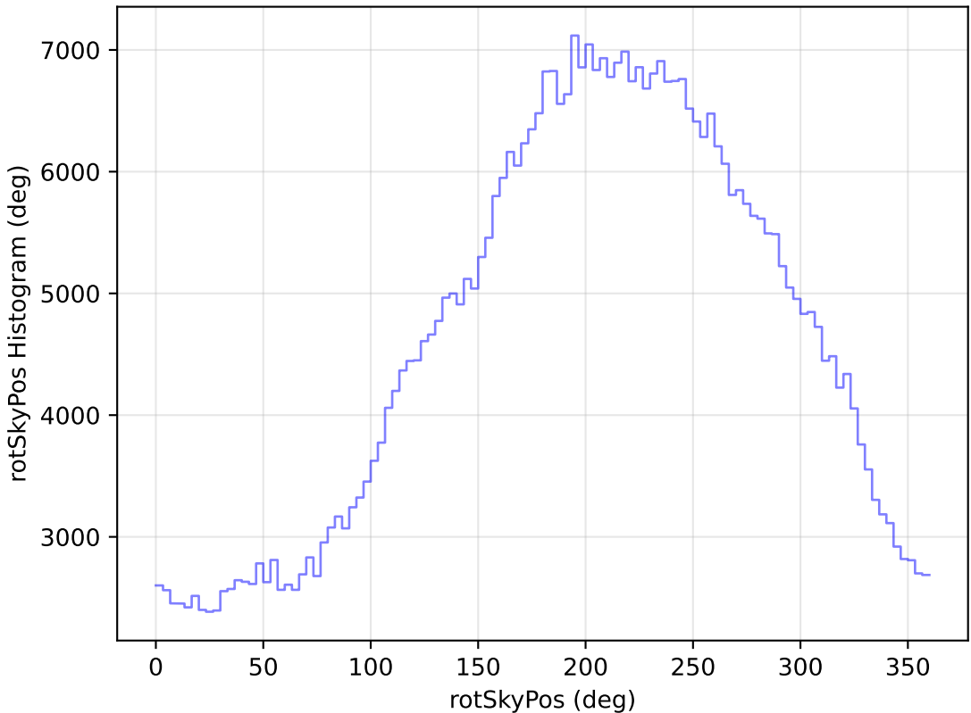
ddf_loaded_half_fl15_v3.4_10yrs WFD i band: rotSkyPos Histogram
