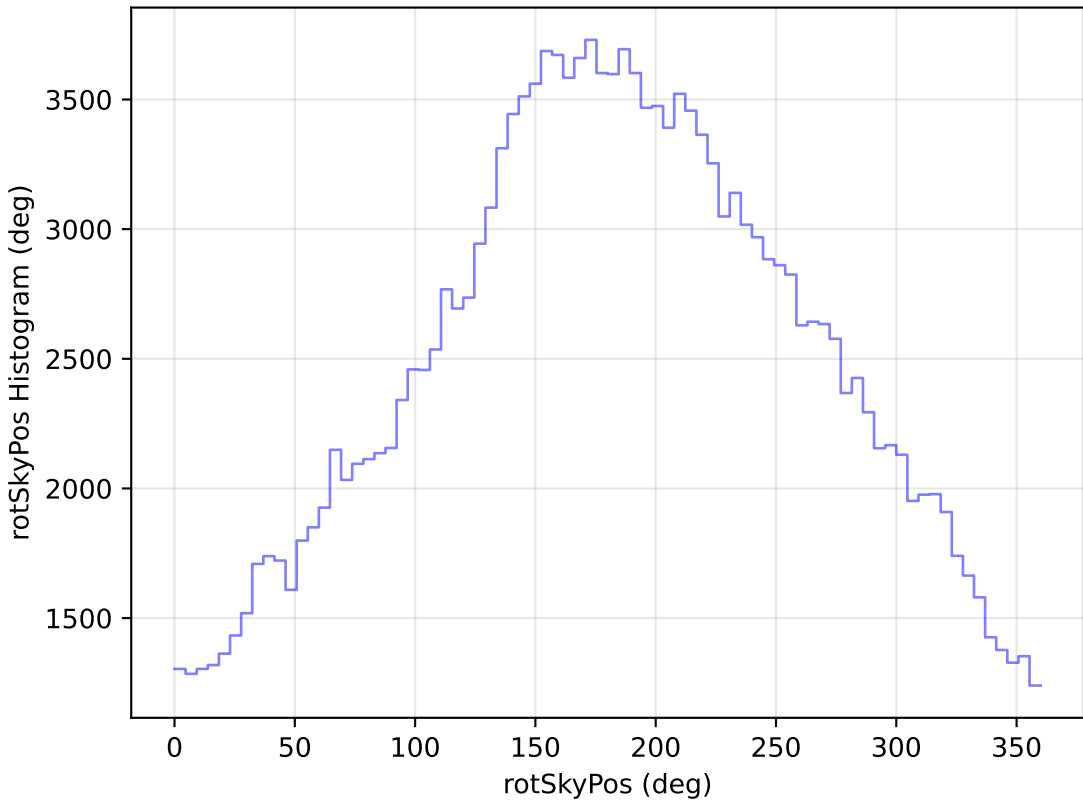
ddf_loaded_half_fl15_v3.4_10yrs WFD g band: rotSkyPos Histogram
