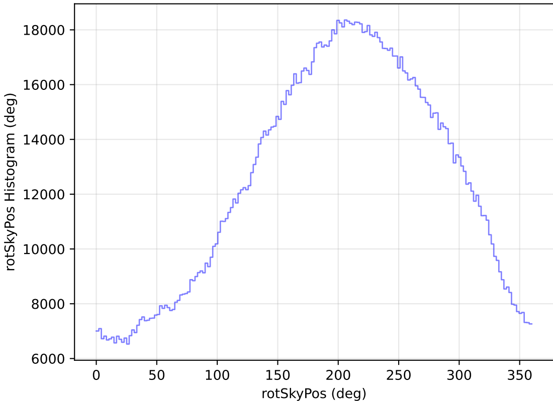
ddf_loaded_half_fl15_v3.4_10yrs WFD all bands: rotSkyPos Histogram
