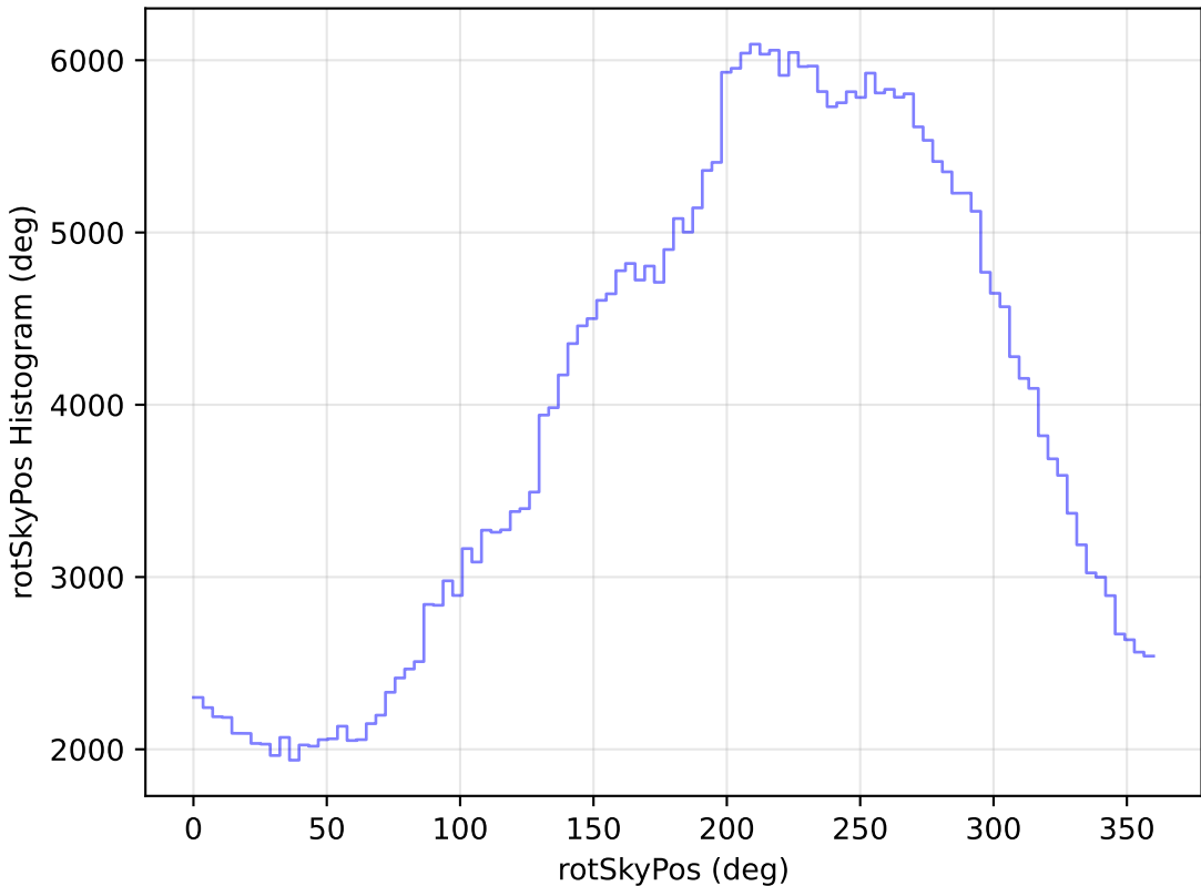
ddf_loaded_half_fl15_v3.4_10yrs All sky y band: rotSkyPos Histogram
