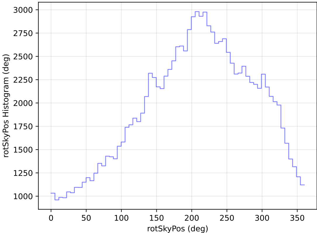
ddf_loaded_half_fl15_v3.4_10yrs All sky u band: rotSkyPos Histogram
