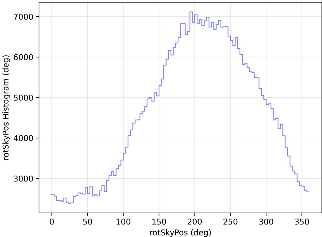
ddf_loaded_half_fl15_v3.4_10yrs All sky i band: rotSkyPos Histogram
