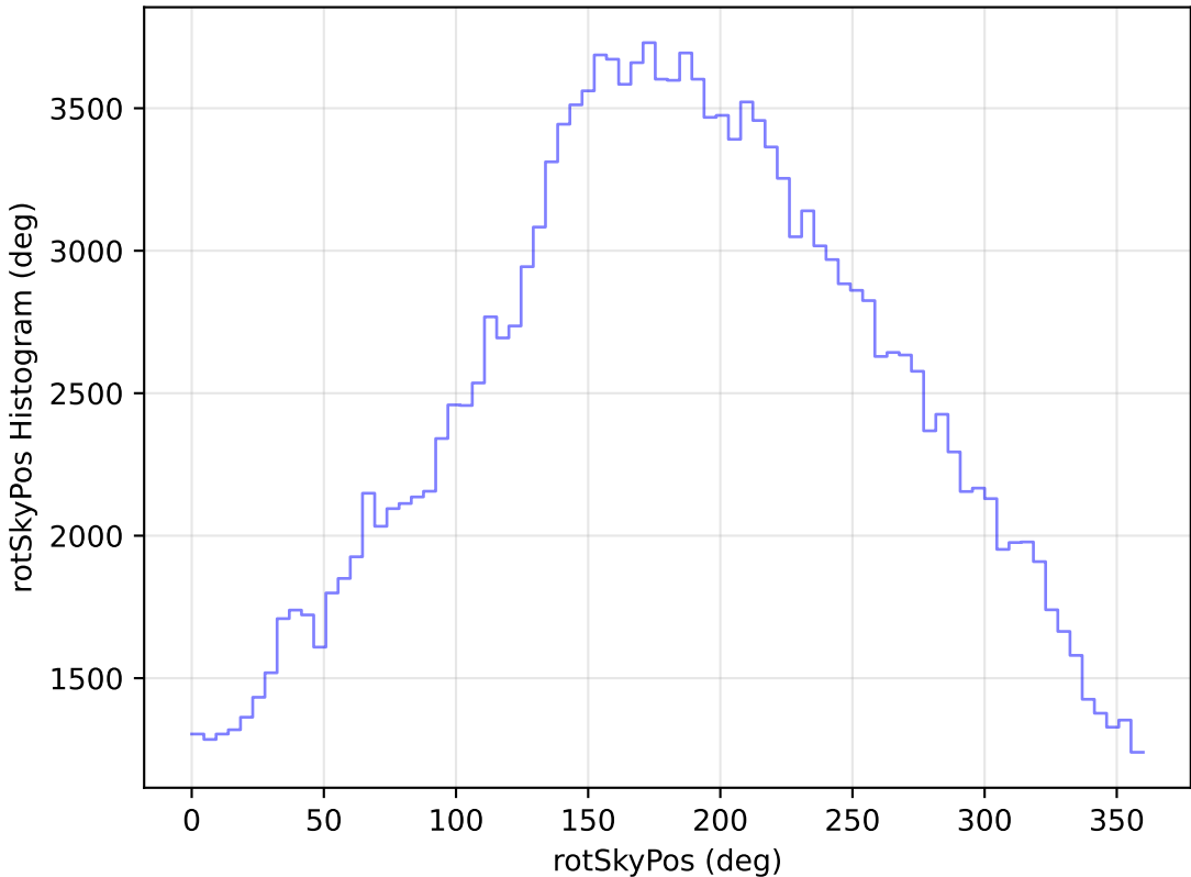
ddf_loaded_half_fl15_v3.4_10yrs All sky g band: rotSkyPos Histogram
