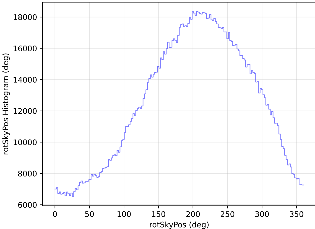
ddf_loaded_half_fl15_v3.4_10yrs All sky all bands: rotSkyPos Histogram
