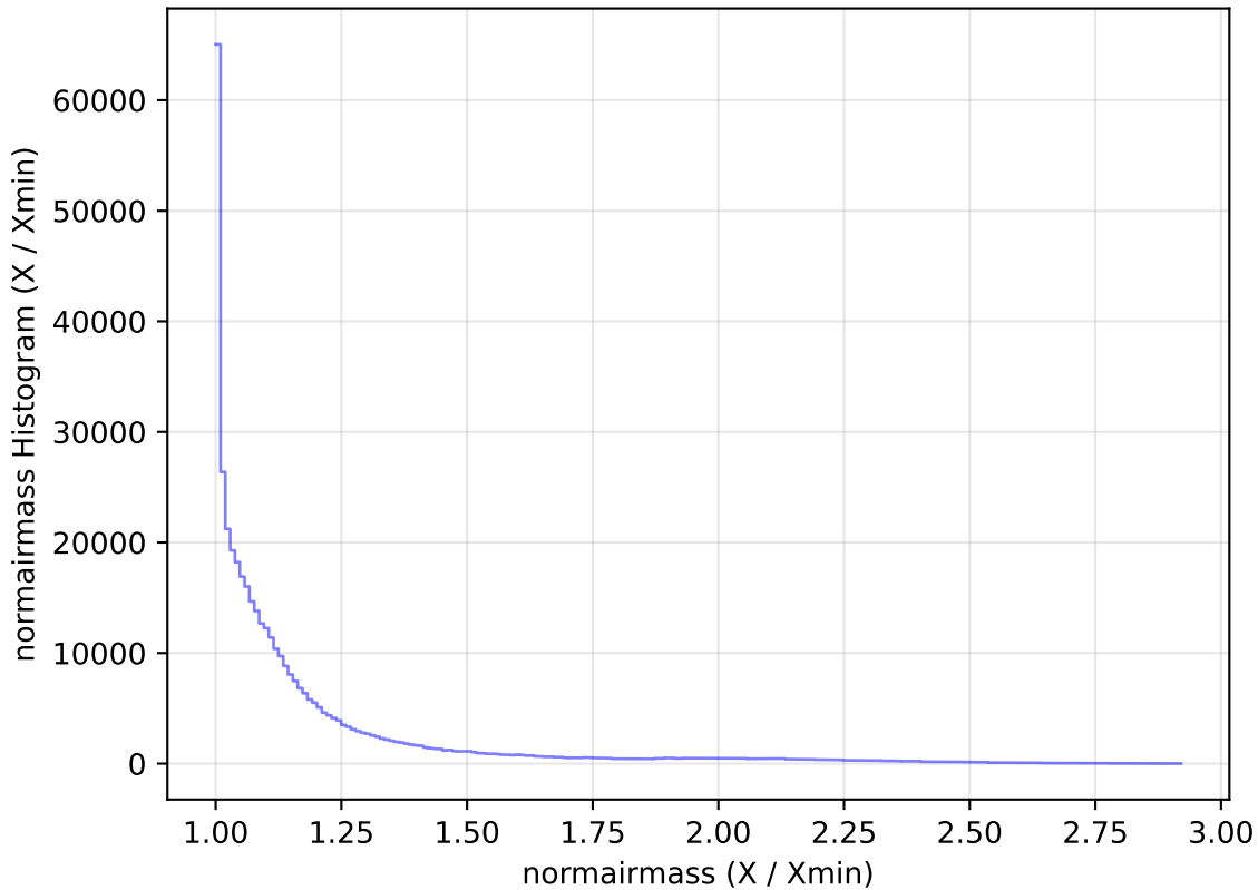
ddf_loaded_half_fl15_v3.4_10yrs WFD z band: normairmass Histogram
