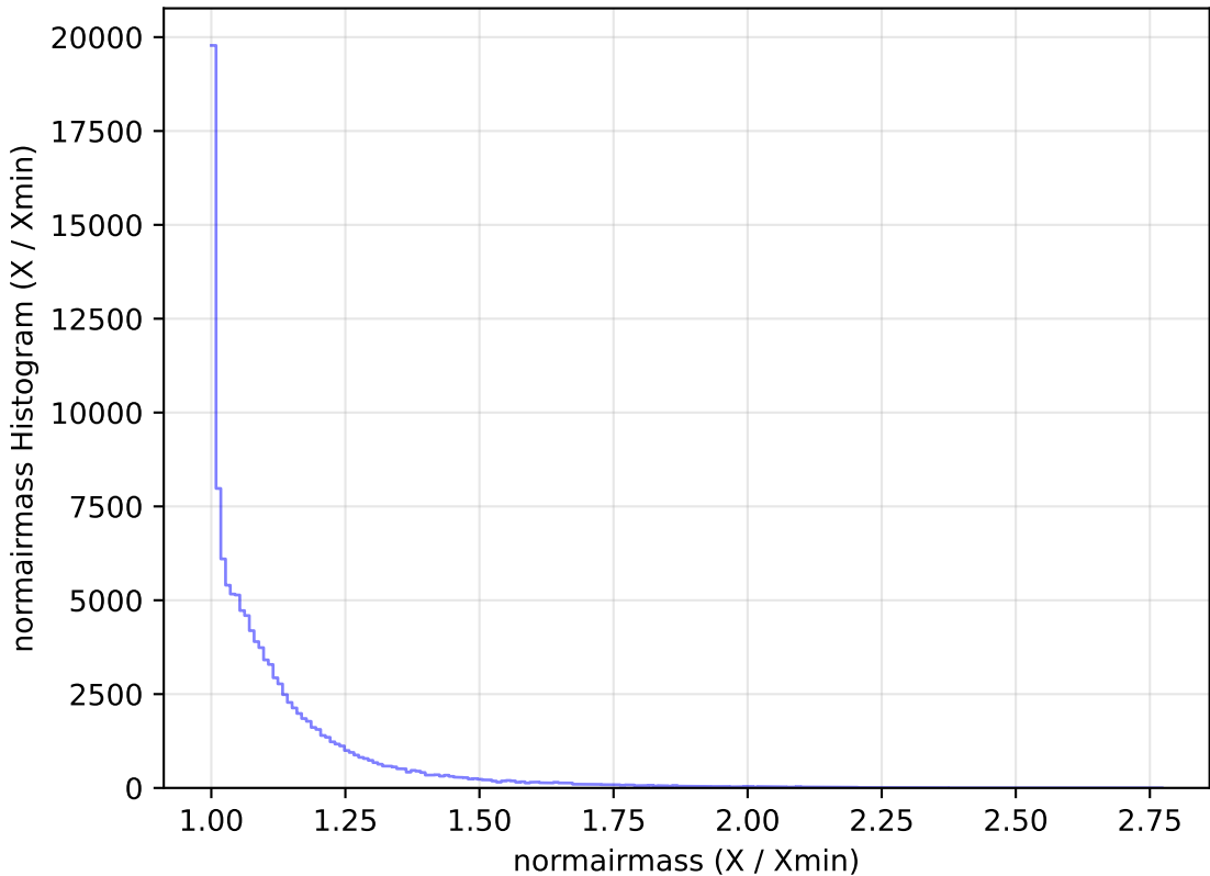
ddf_loaded_half_fl15_v3.4_10yrs WFD u band: normairmass Histogram
