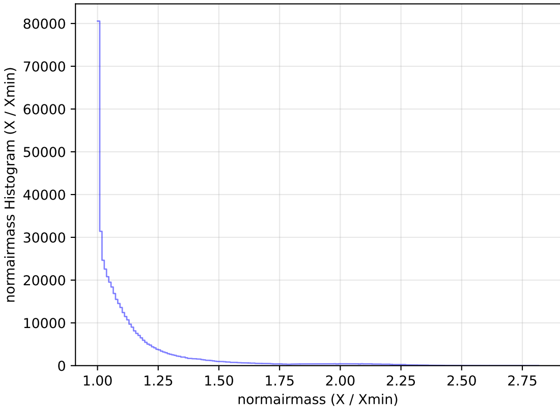
ddf_loaded_half_fl15_v3.4_10yrs WFD r band: normairmass Histogram
