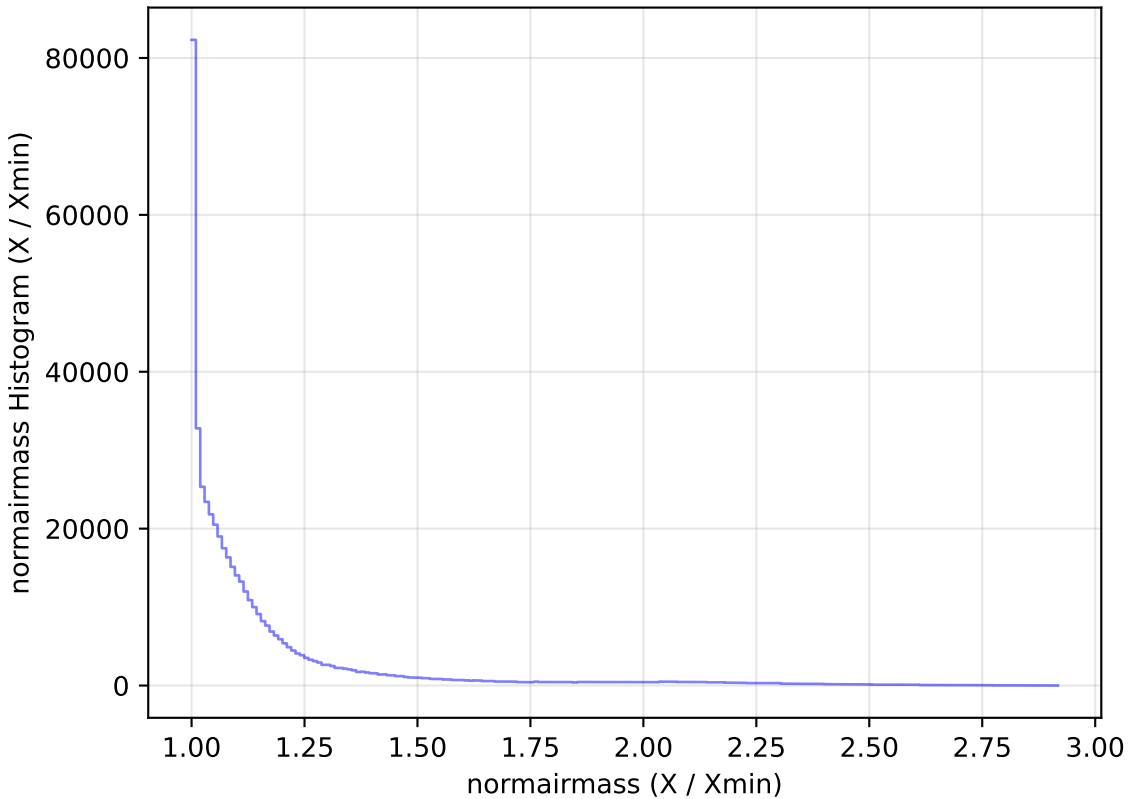
ddf_loaded_half_fl15_v3.4_10yrs WFD i band: normairmass Histogram
