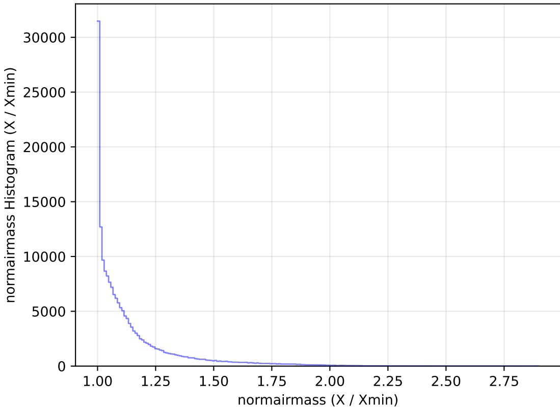
ddf_loaded_half_fl15_v3.4_10yrs WFD g band: normairmass Histogram
