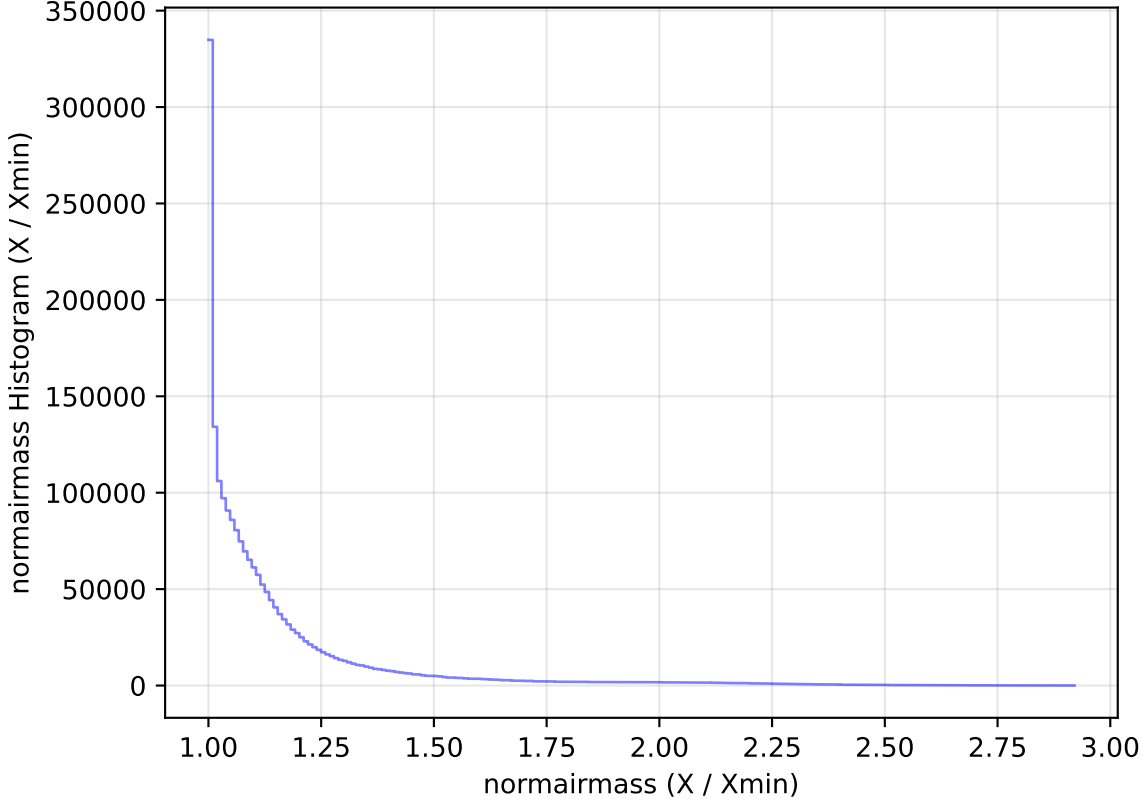
ddf_loaded_half_fl15_v3.4_10yrs WFD all bands: normairmass Histogram
