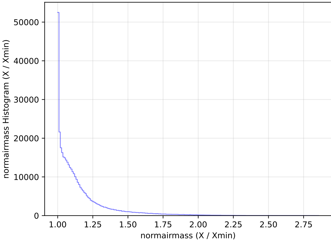
ddf_loaded_half_fl15_v3.4_10yrs All sky y band: normairmass Histogram
