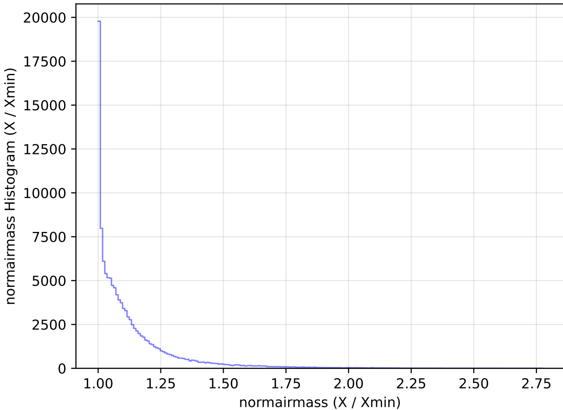
ddf_loaded_half_fl15_v3.4_10yrs All sky u band: normairmass Histogram
