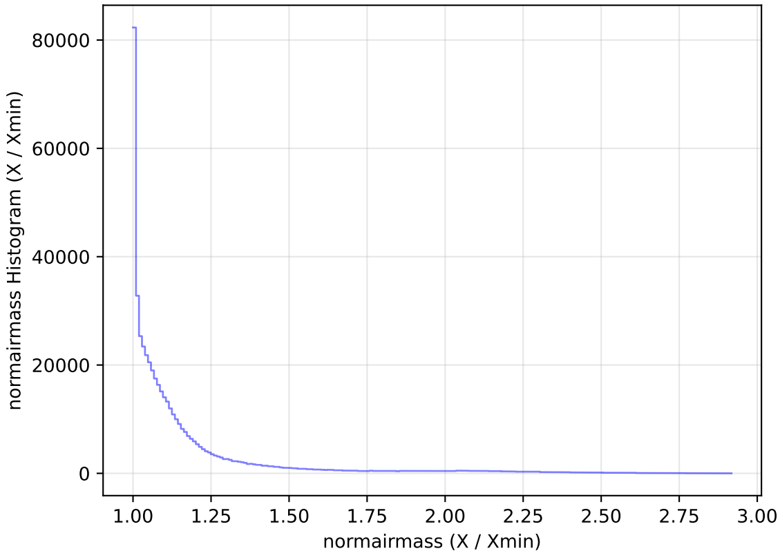
ddf_loaded_half_fl15_v3.4_10yrs All sky i band: normairmass Histogram
