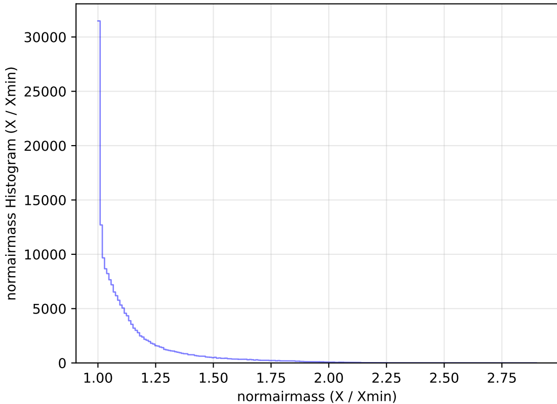
ddf_loaded_half_fl15_v3.4_10yrs All sky g band: normairmass Histogram
