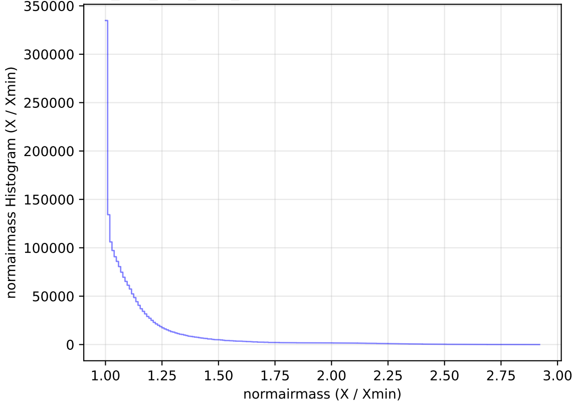
ddf_loaded_half_fl15_v3.4_10yrs All sky all bands: normairmass Histogram
