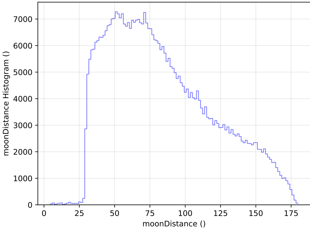
ddf_loaded_half_fl15_v3.4_10yrs WFD z band: moonDistance Histogram
