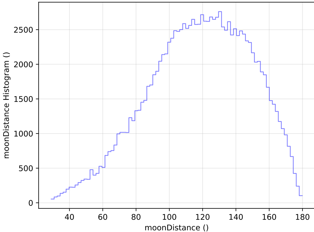
ddf_loaded_half_fl15_v3.4_10yrs WFD u band: moonDistance Histogram
