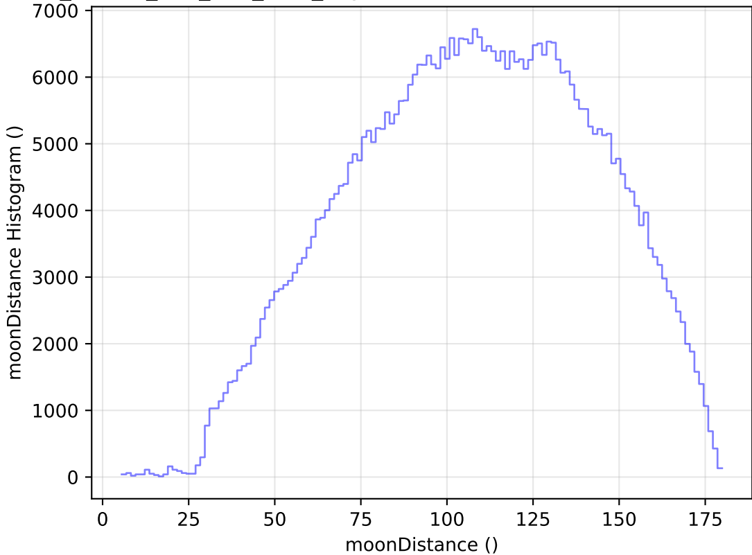
ddf_loaded_half_fl15_v3.4_10yrs WFD r band: moonDistance Histogram
