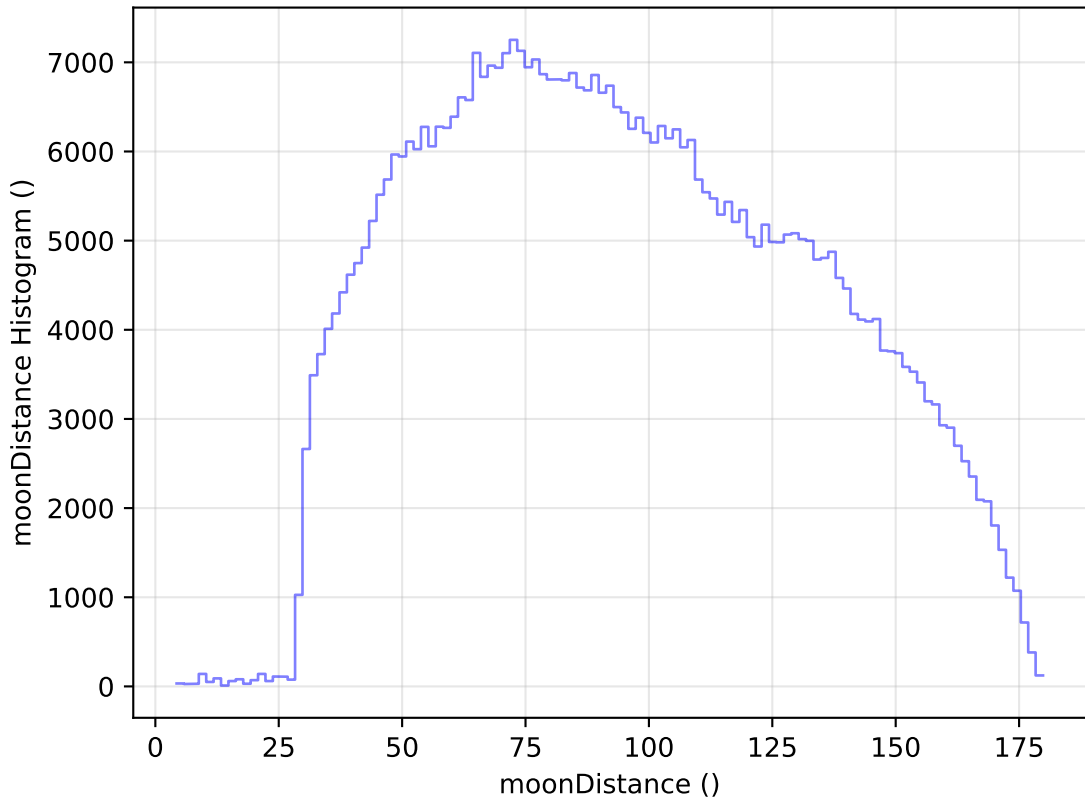
ddf_loaded_half_fl15_v3.4_10yrs WFD i band: moonDistance Histogram
