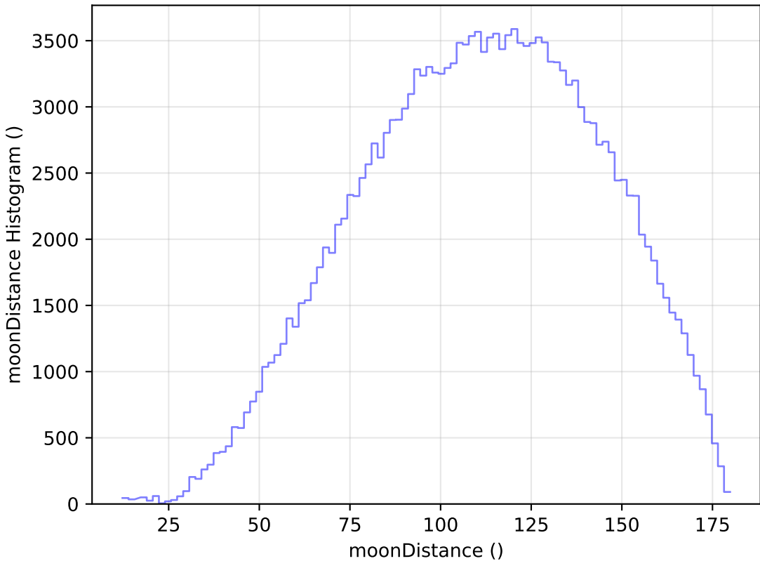
ddf_loaded_half_fl15_v3.4_10yrs WFD g band: moonDistance Histogram
