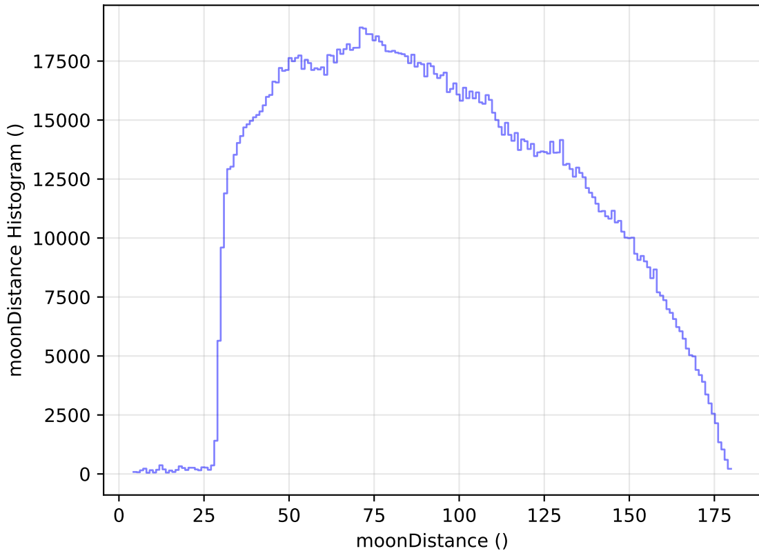
ddf_loaded_half_fl15_v3.4_10yrs WFD all bands: moonDistance Histogram
