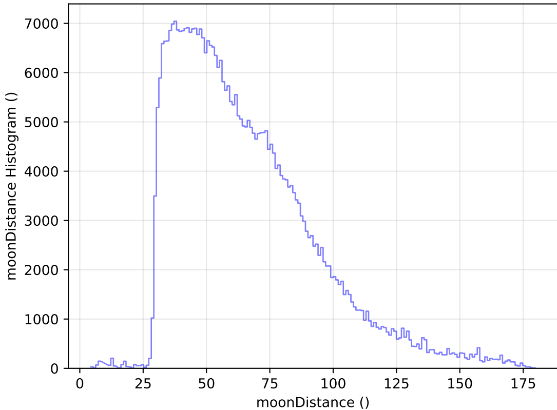
ddf_loaded_half_fl15_v3.4_10yrs All sky y band: moonDistance Histogram
