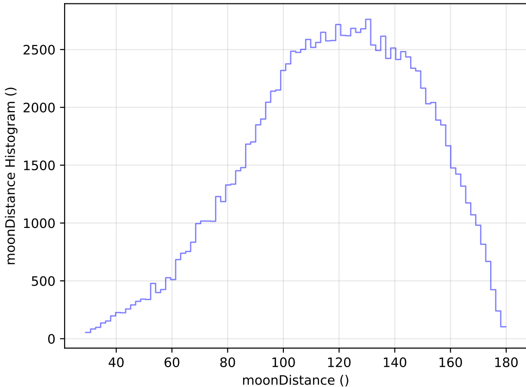
ddf_loaded_half_fl15_v3.4_10yrs All sky u band: moonDistance Histogram
