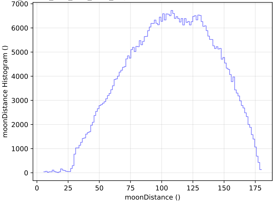
ddf_loaded_half_fl15_v3.4_10yrs All sky r band: moonDistance Histogram
