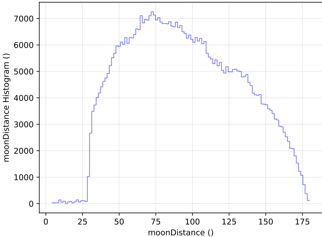
ddf_loaded_half_fl15_v3.4_10yrs All sky i band: moonDistance Histogram
